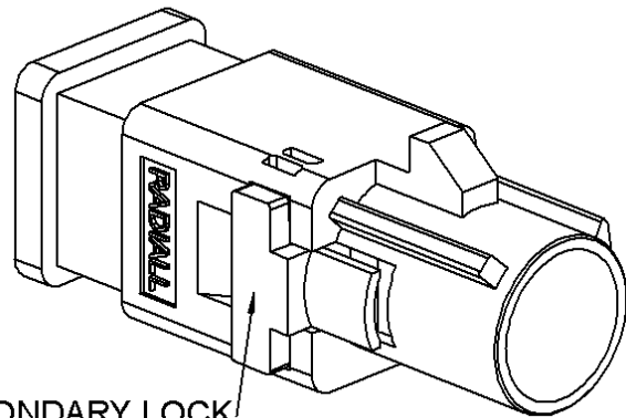
SECONDARY LOCK
